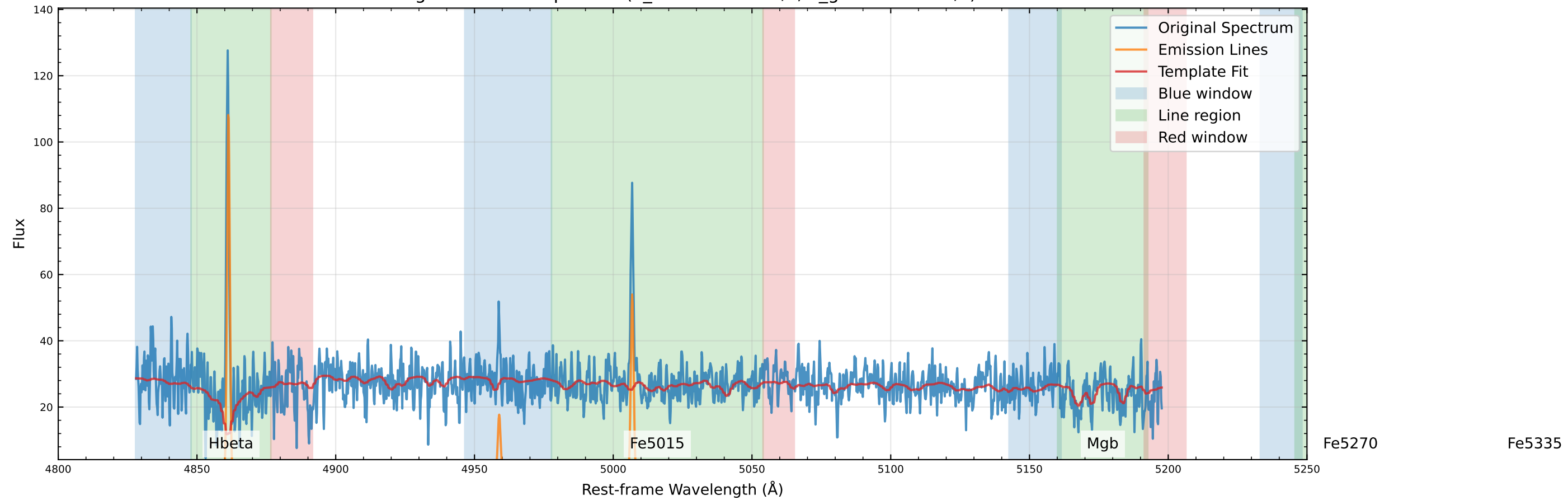
Original Data Comparison (v_star=-15.1 km/s, v_gas=-15.1 km/s)
