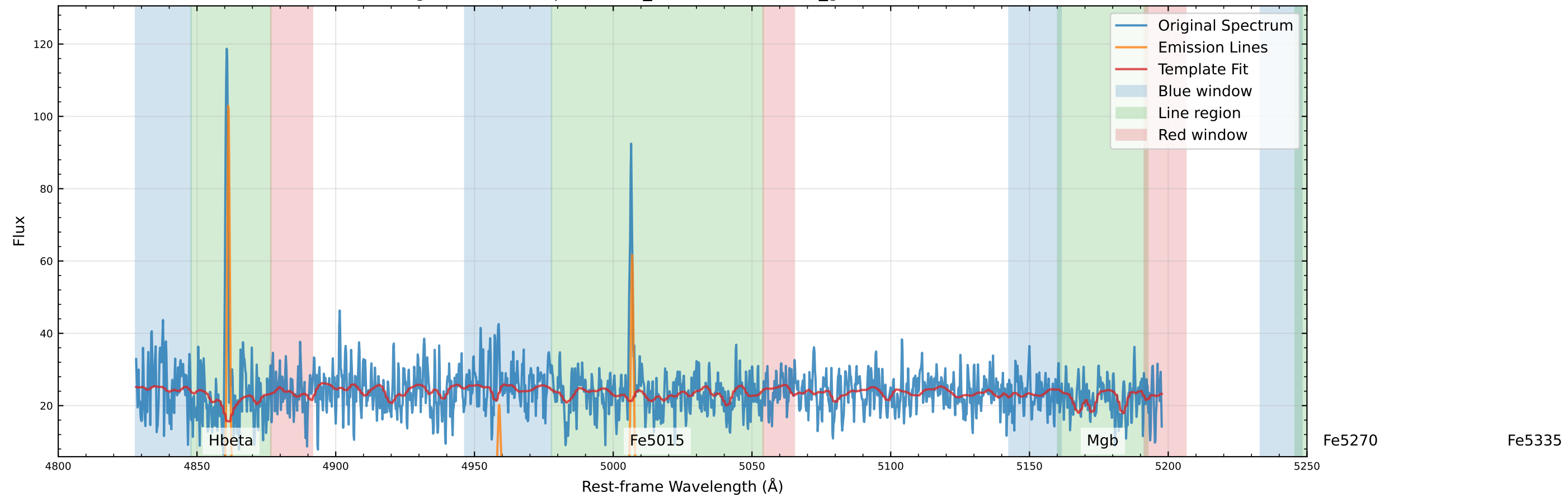
Original Data Comparison (v_star=-13.0 km/s, v_gas=-34.1 km/s)
