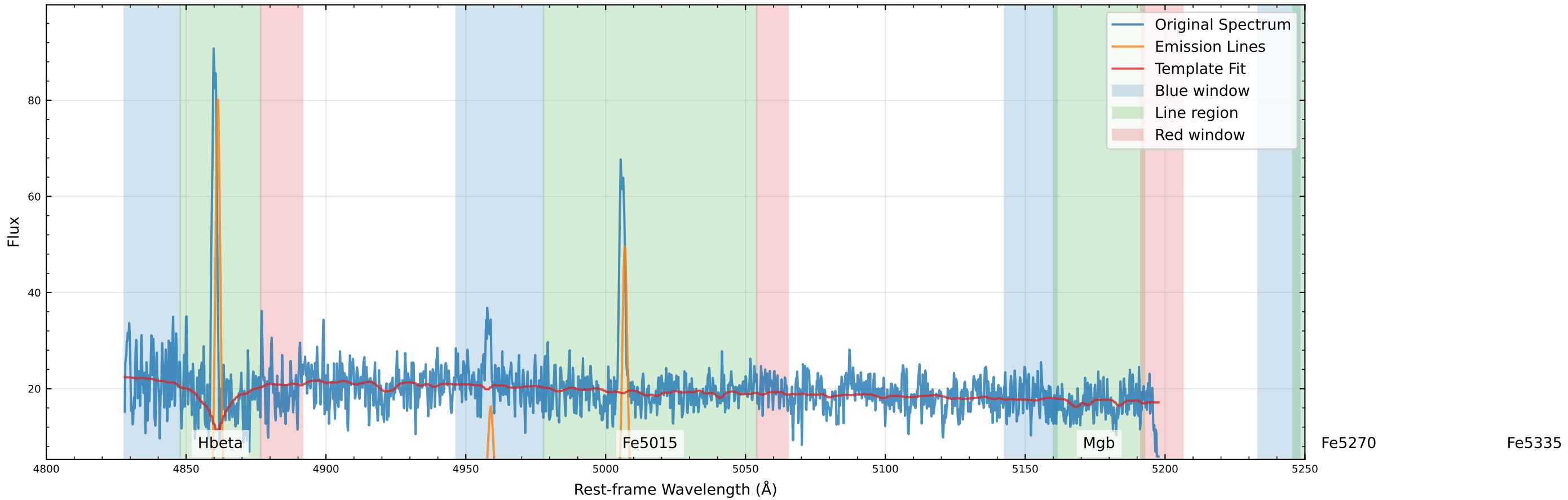
Original Data Comparison (v_star=-106.0 km/s, v_gas=-69.8 km/s)
