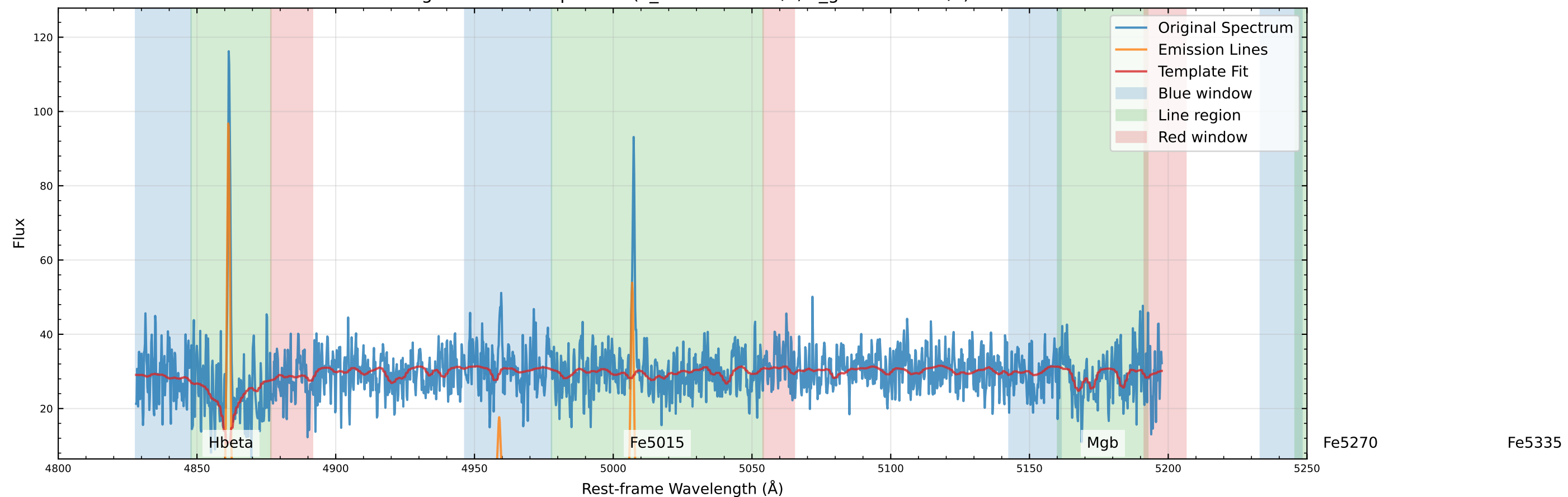
Original Data Comparison (v_star=29.9 km/s, v_gas=19.7 km/s)
