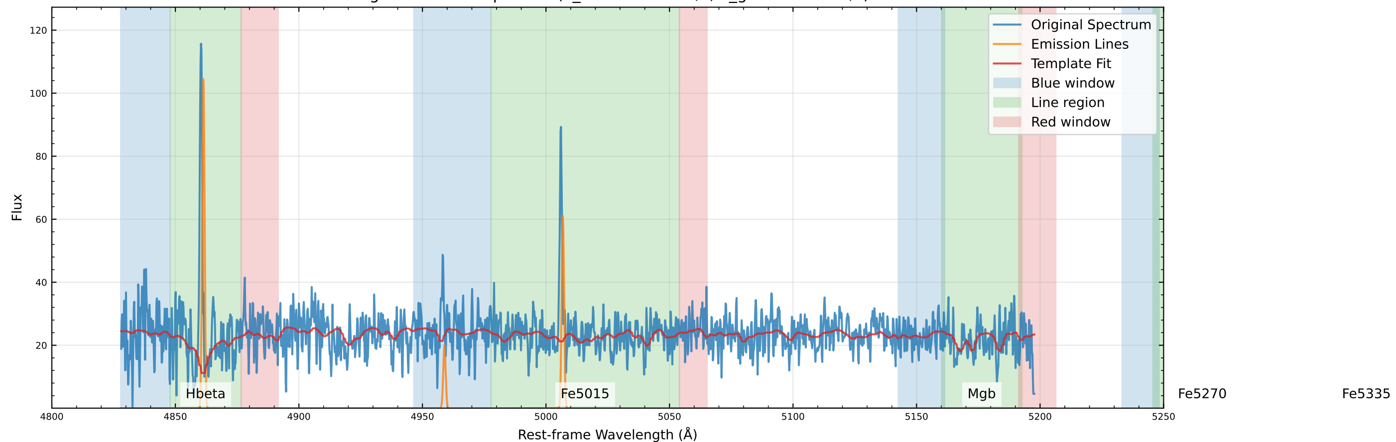
Original Data Comparison (v_star=-56.6 km/s, v_gas=-57.2 km/s)
