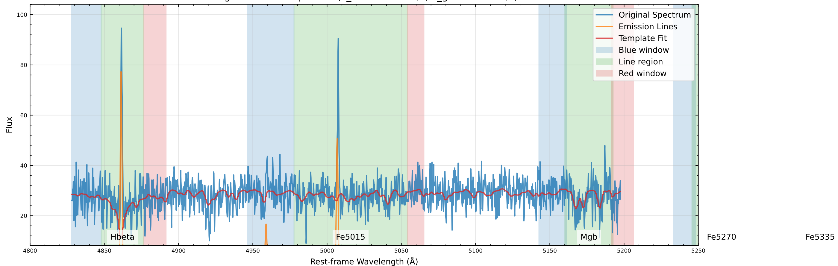
Original Data Comparison (v_star=27.6 km/s, v_gas=24.6 km/s)
