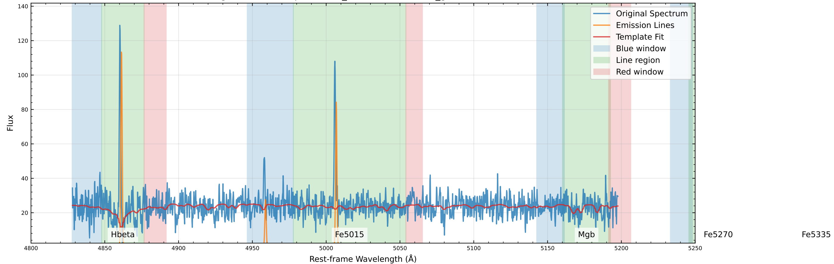
Original Data Comparison (v_star=-70.7 km/s, v_gas=-61.1 km/s)
