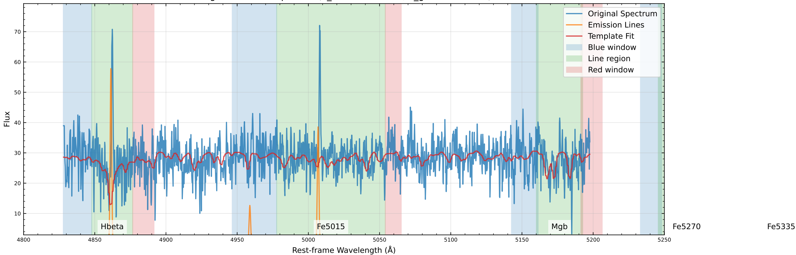
Original Data Comparison (v_star=65.0 km/s, v_gas=65.8 km/s)
