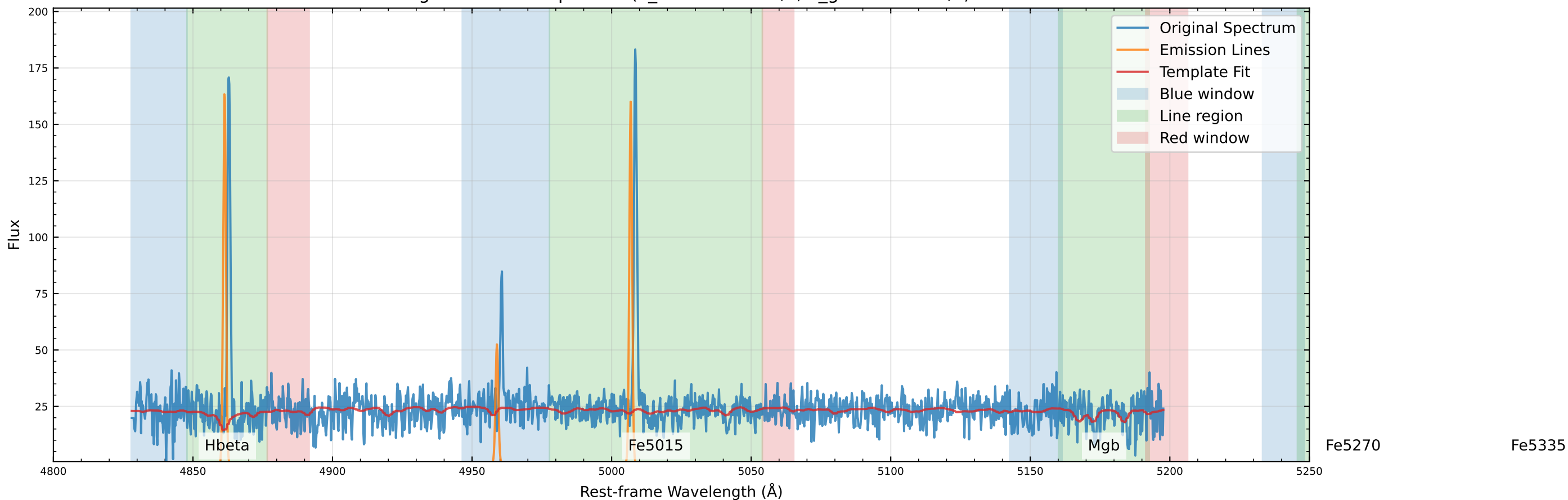
Original Data Comparison (v_star=91.4 km/s, v_gas=97.4 km/s)
