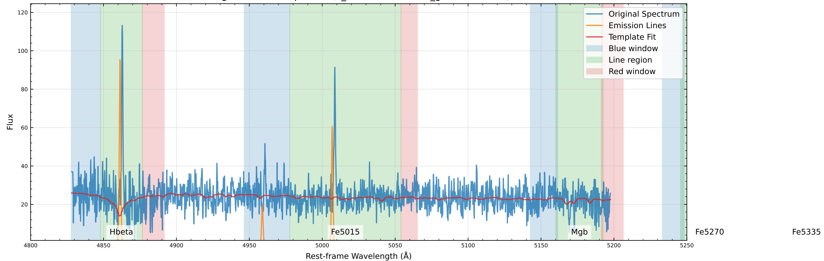
Original Data Comparison (v_star=99.5 km/s, v_gas=97.5 km/s)
