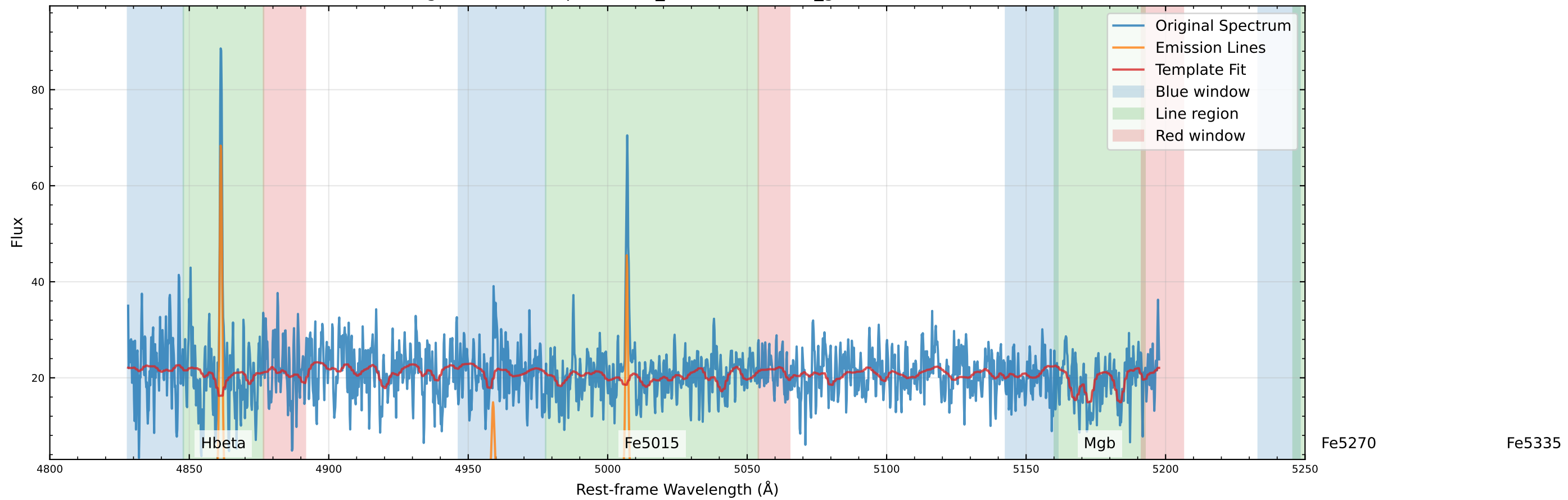
Original Data Comparison ( v_{\text{star}}=8.9 km/s, v_{\text{gas}}=5.8 km/s)
