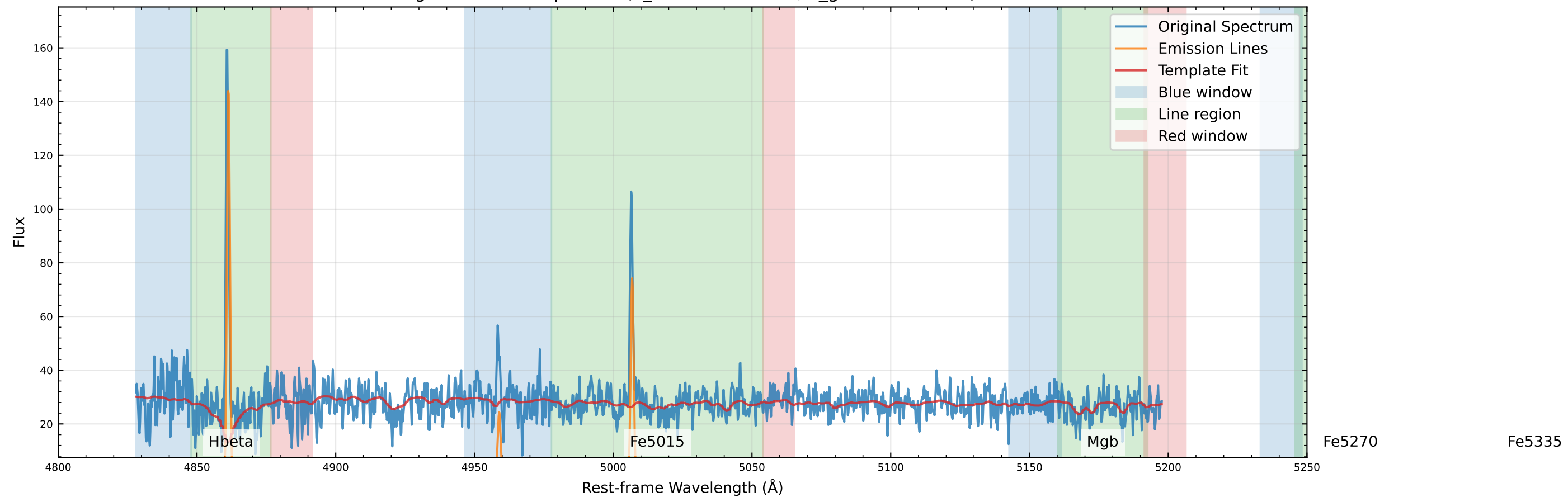
Original Data Comparison (v_star=-25.9 km/s, v_gas=-23.3 km/s)
