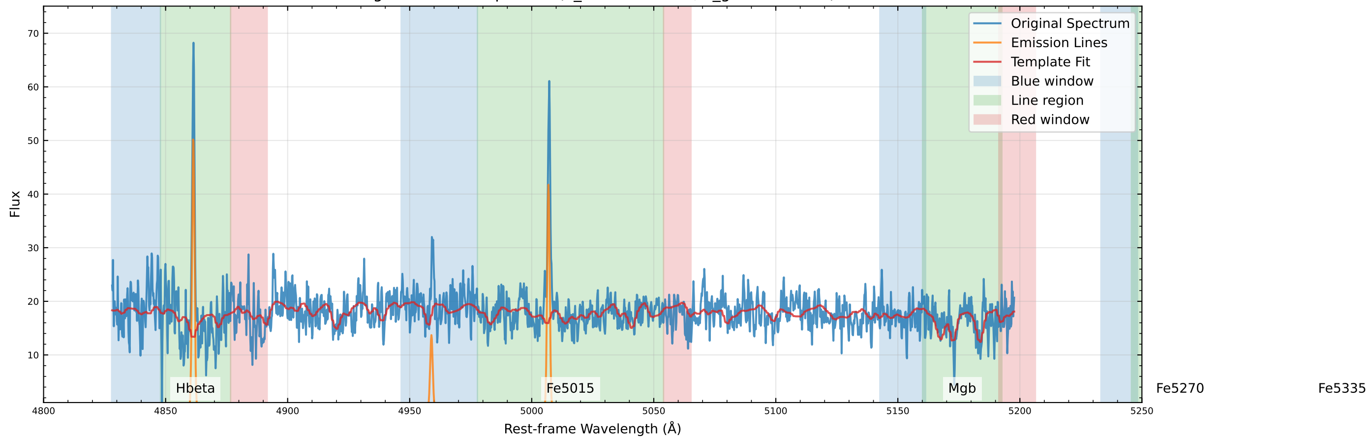
Original Data Comparison (v_star=1.3 km/s, v_gas=8.0 km/s)
