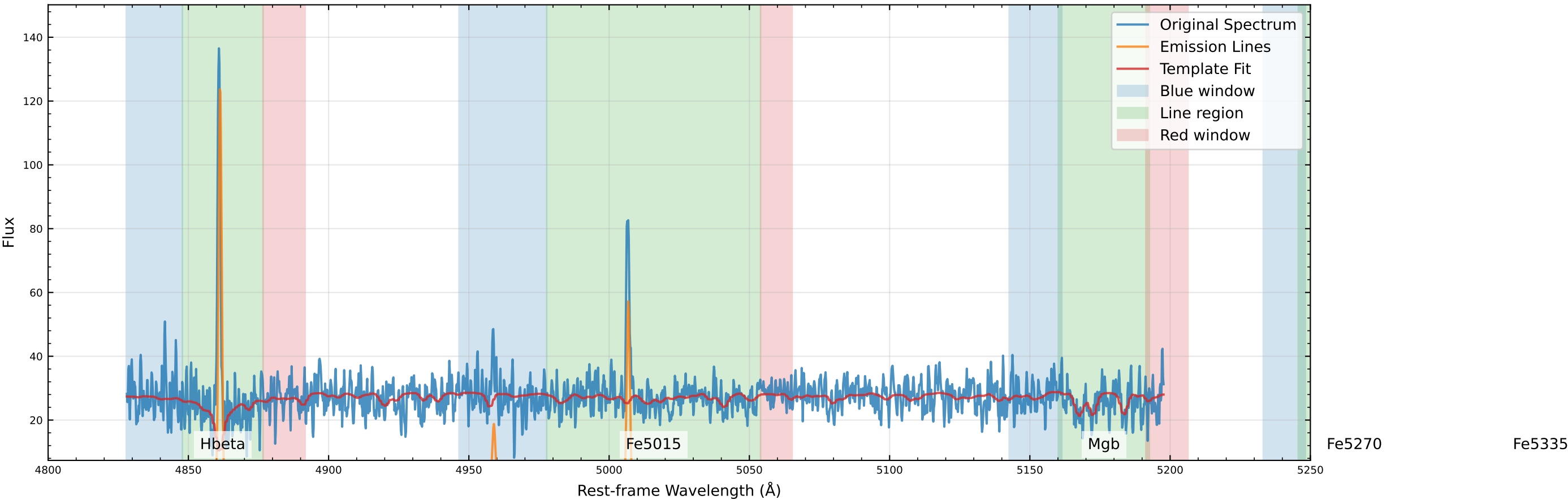
Original Data Comparison (v_star=-10.4 km/s, v_gas=-24.2 km/s)
