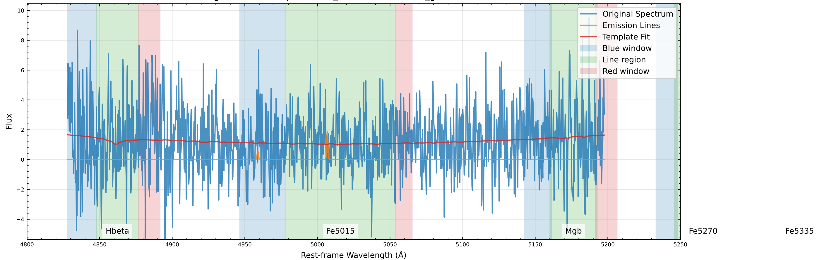
Original Data Comparison ( v_{\text{star}}=-71.1 km/s, v_{\text{gas}}=-86.9 km/s)
