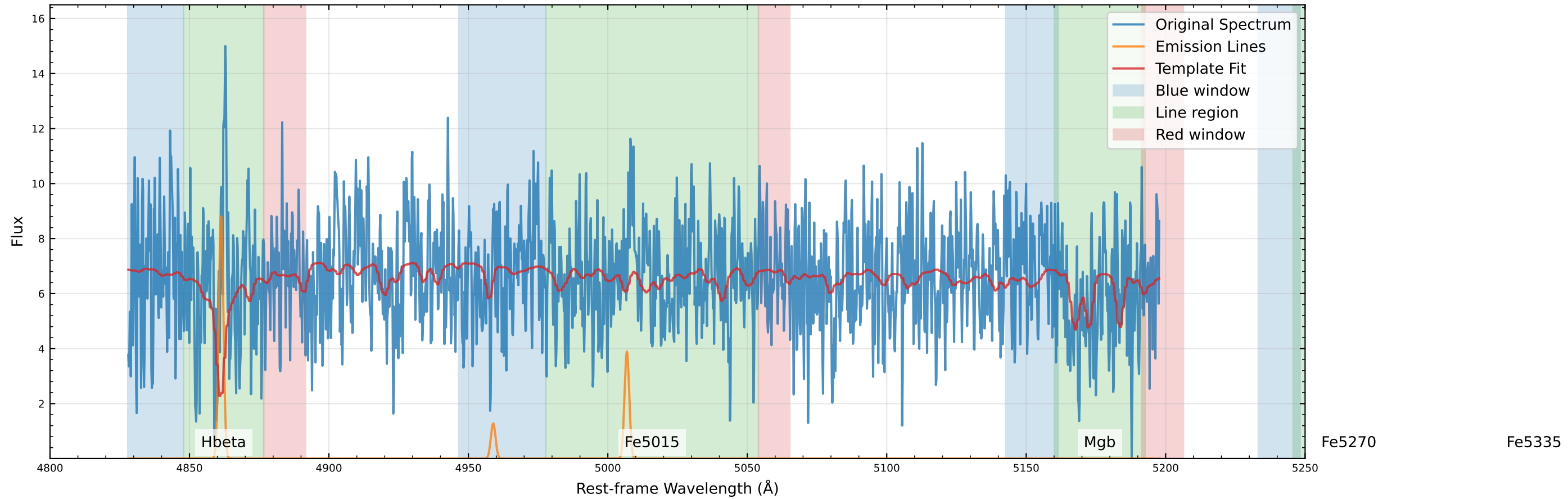
Original Data Comparison (v_star=10.5 km/s, v_gas=80.5 km/s)
