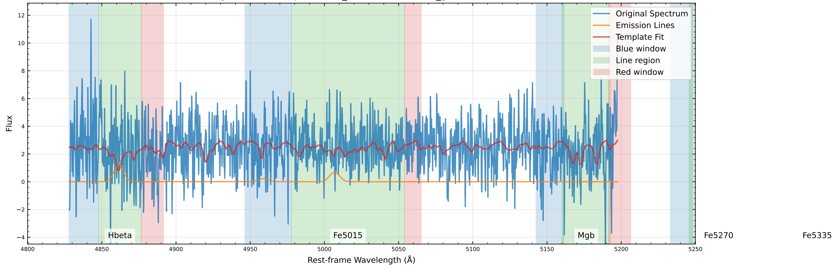
Original Data Comparison (v_star=-68.6 km/s, v_gas=12.6 km/s)
