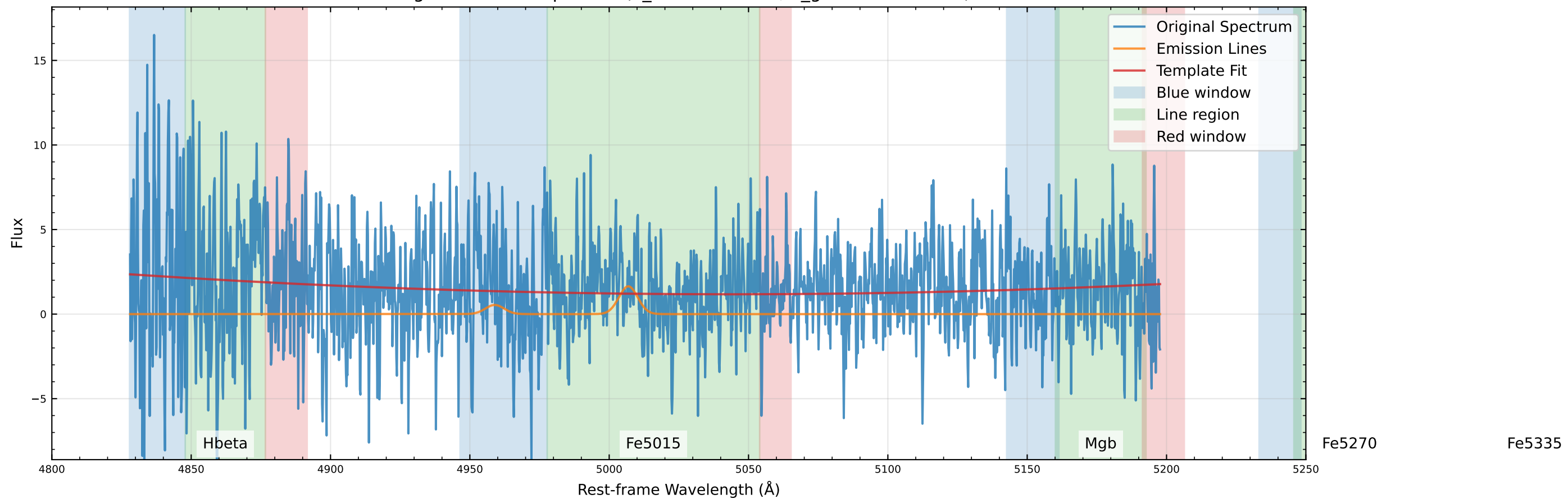
Original Data Comparison (v_star=0.0 km/s, v_gas=-268.1 km/s)
