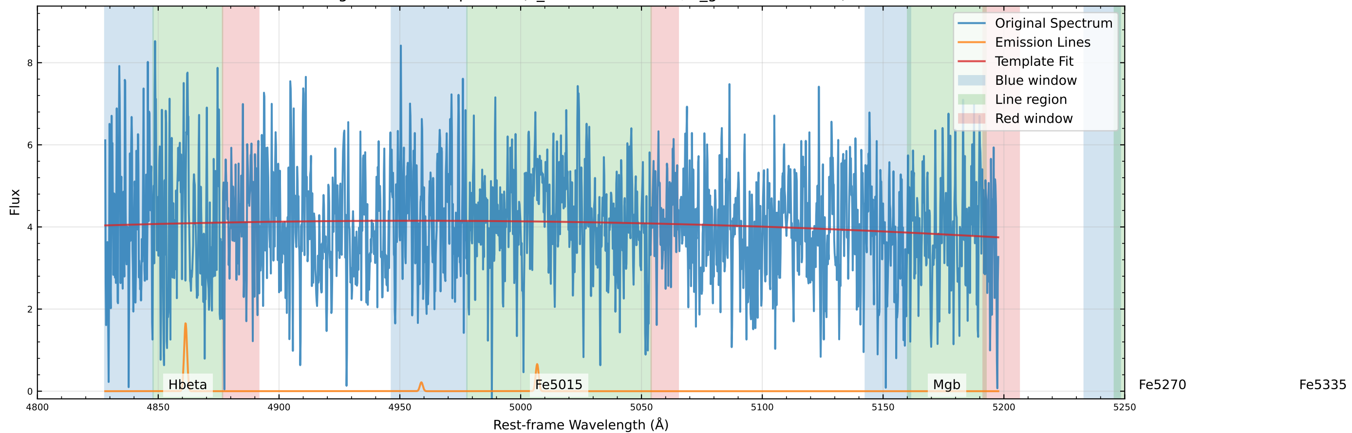
Original Data Comparison (v_star=-219.3 km/s, v_gas=-164.1 km/s)
