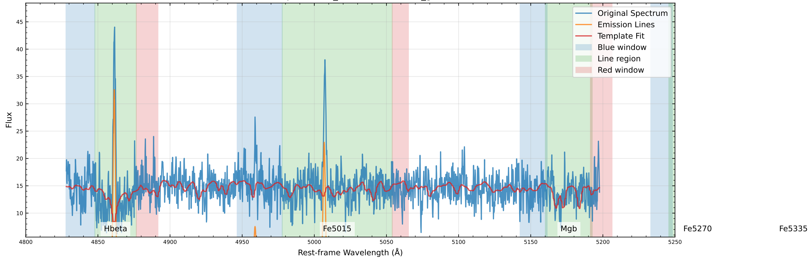
Original Data Comparison (v_star=11.5 km/s, v_gas=13.6 km/s)
