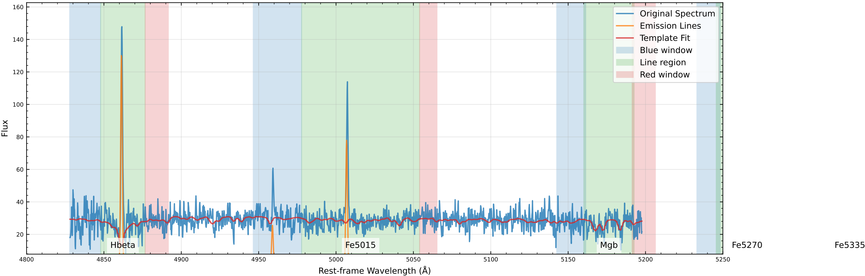
Original Data Comparison (v_star=27.2 km/s, v_gas=19.2 km/s)
