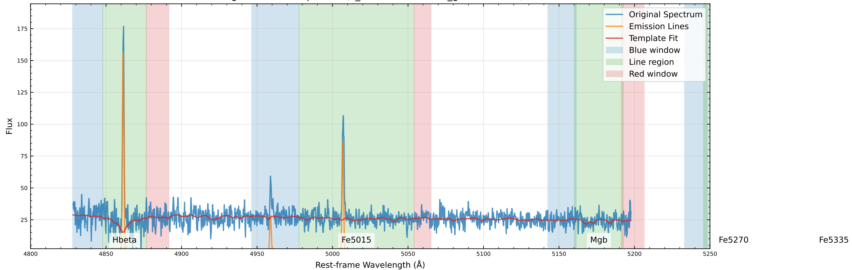
Original Data Comparison (v_star=24.1 km/s, v_gas=7.6 km/s)
