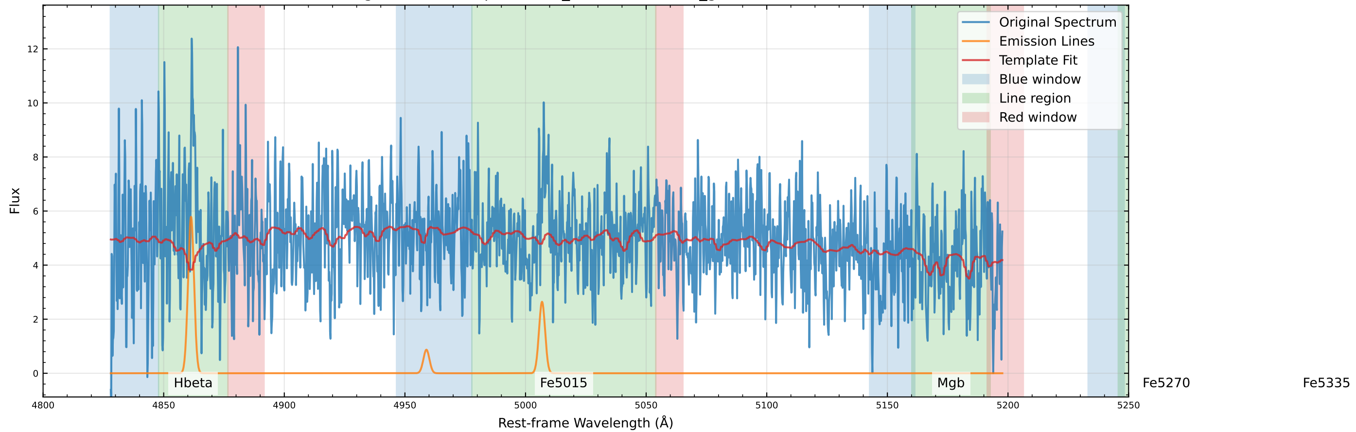
Original Data Comparison (v_star=8.2 km/s, v_gas=46.5 km/s)
