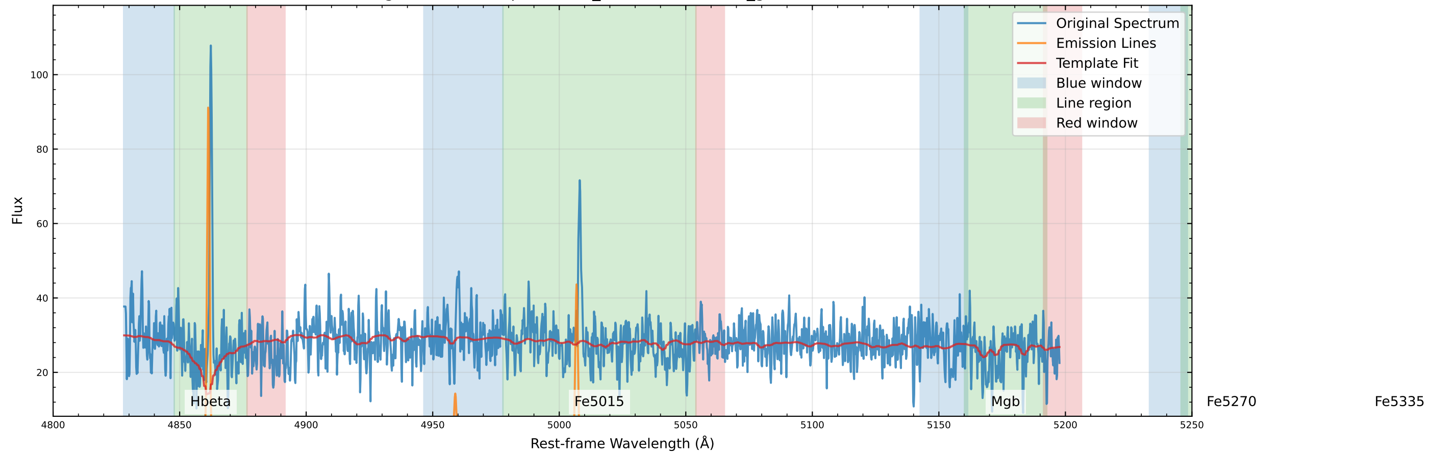
Original Data Comparison (v_star=79.8 km/s, v_gas=64.8 km/s)
