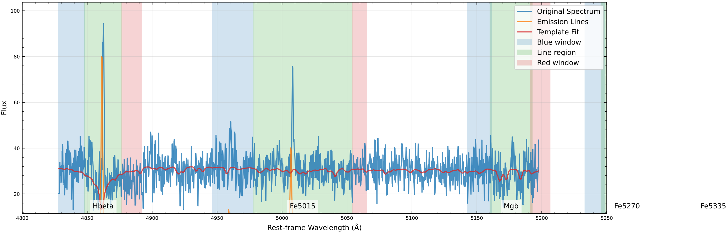
Original Data Comparison (v_star=90.4 km/s, v_gas=71.7 km/s)
