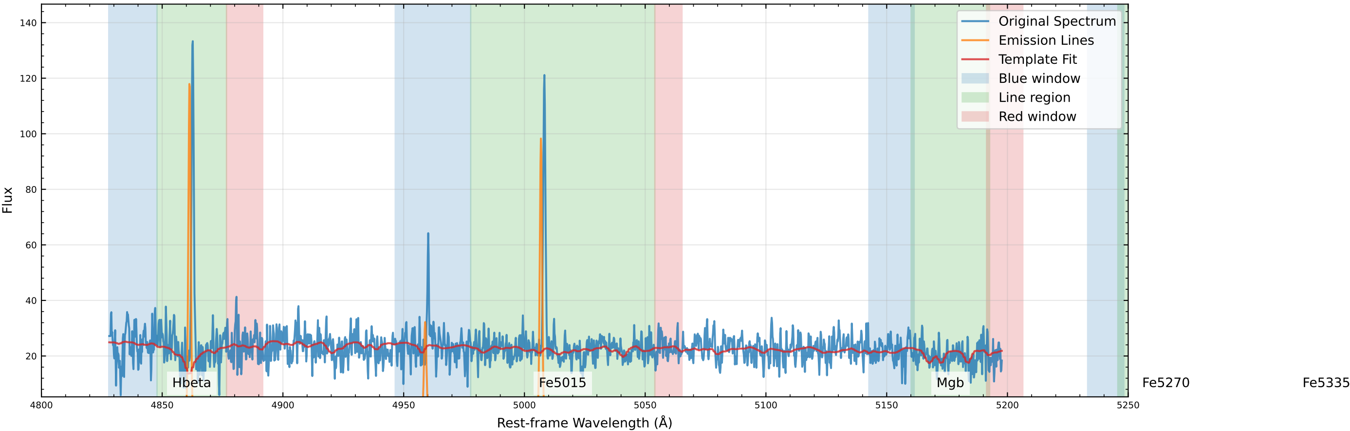
Original Data Comparison (v_star=74.1 km/s, v_gas=80.3 km/s)
