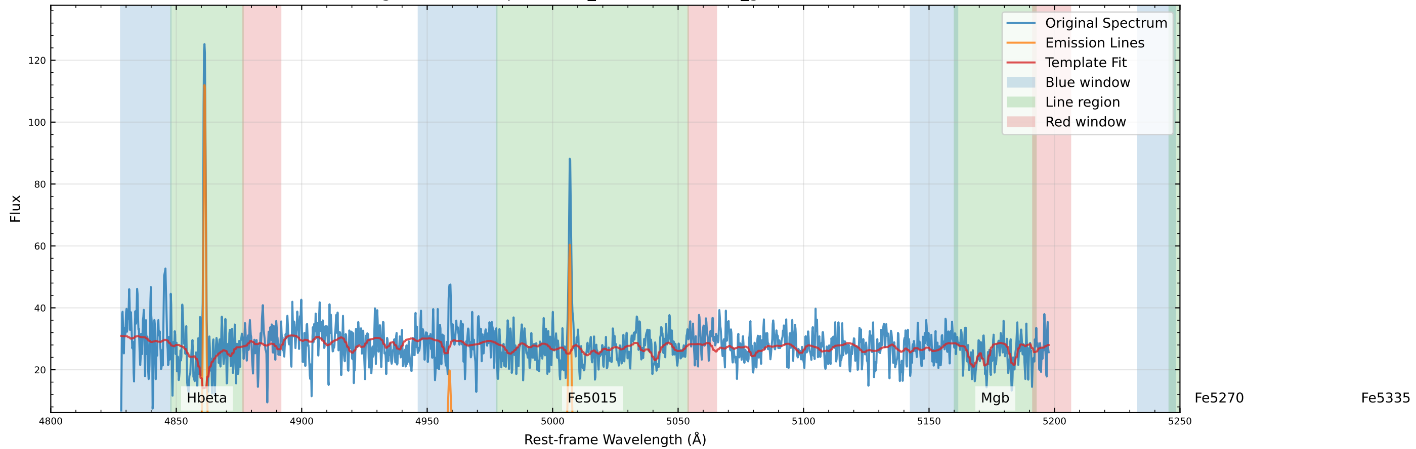
Original Data Comparison (v_star=10.6 km/s, v_gas=-1.3 km/s)
