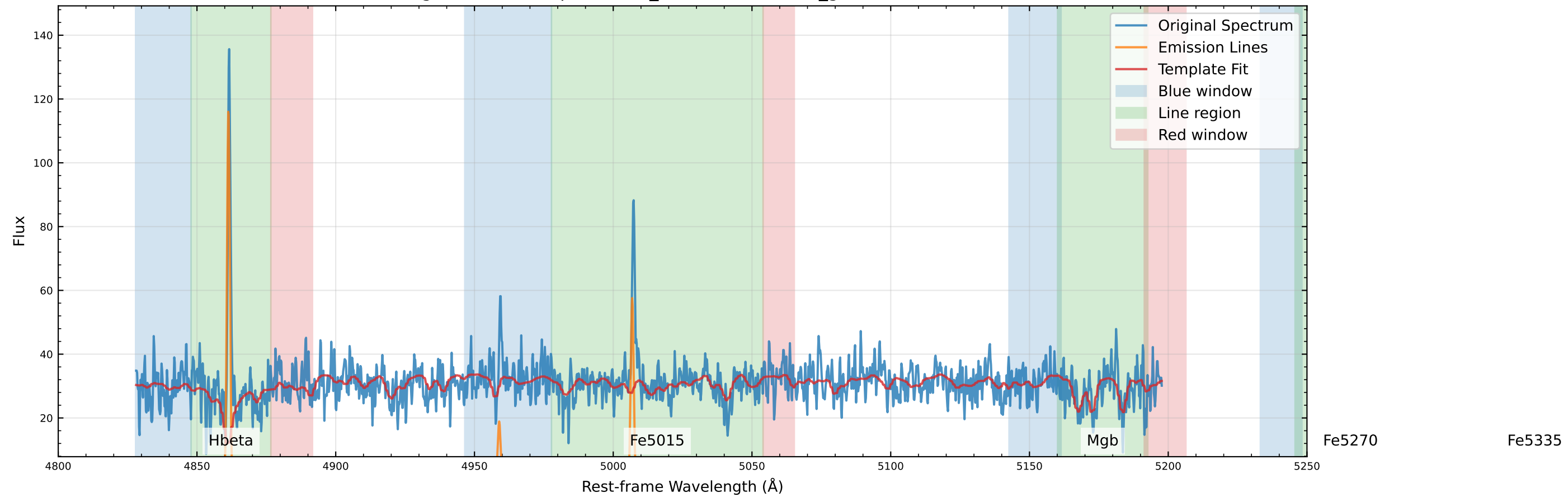
Original Data Comparison (v_star=33.7 km/s, v_gas=20.2 km/s)
