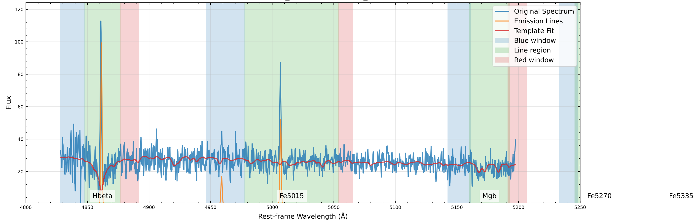
Original Data Comparison (v_star=-30.3 km/s, v_gas=-22.4 km/s)
