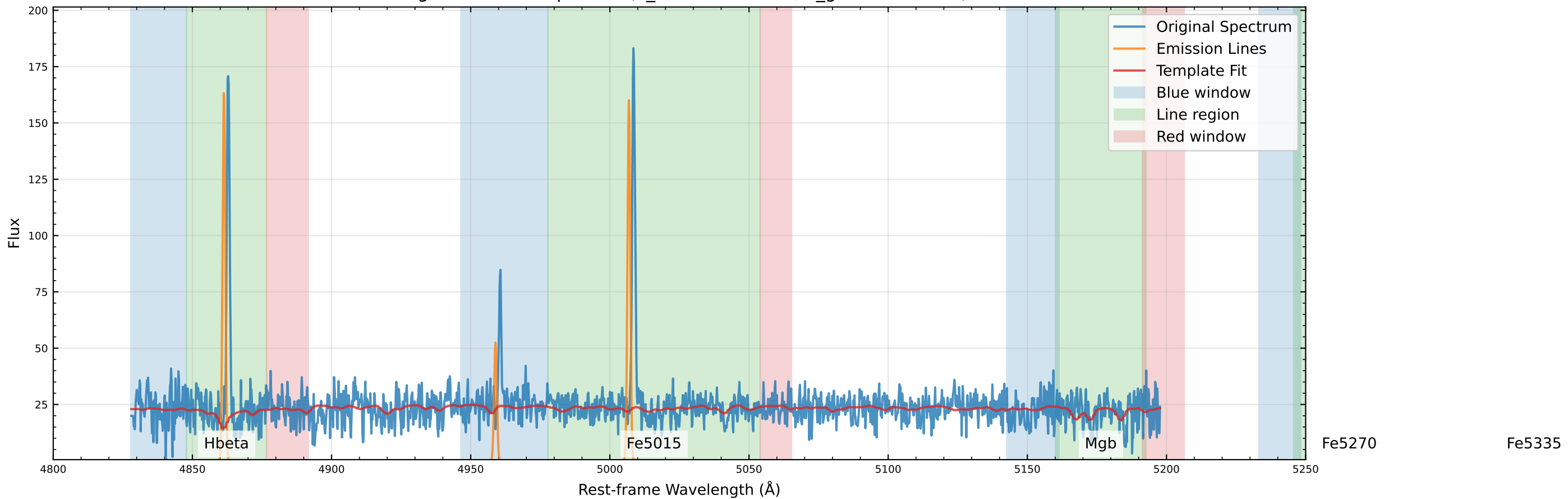
Original Data Comparison ( v_{\text{star}}=91.4 km/s, v_{\text{gas}}=97.4 km/s)
