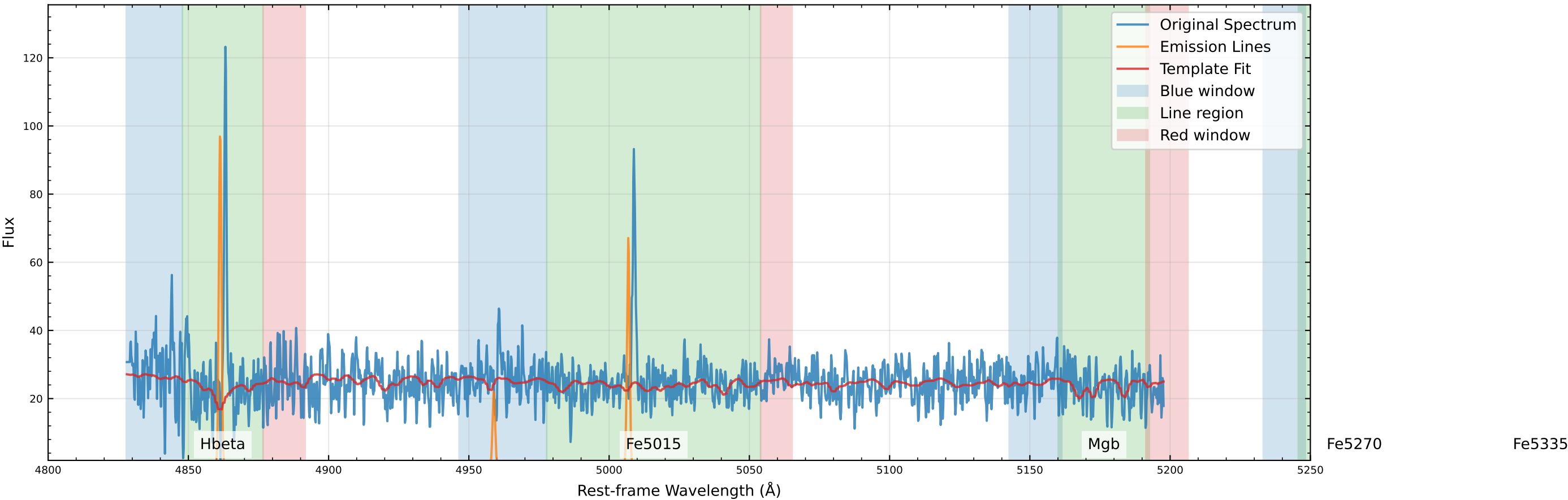
Original Data Comparison (v_star=142.2 km/s, v_gas=117.4 km/s)
