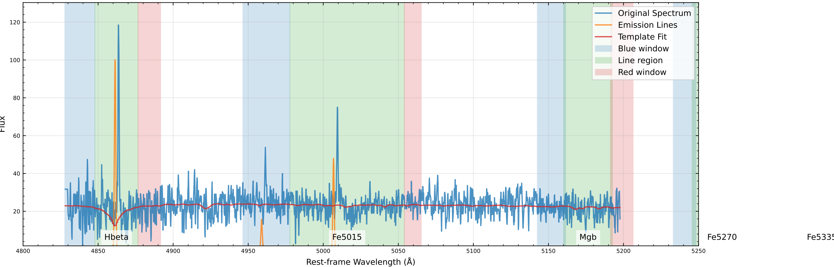
Original Data Comparison (v_star=184.2 km/s, v_gas=145.8 km/s)
