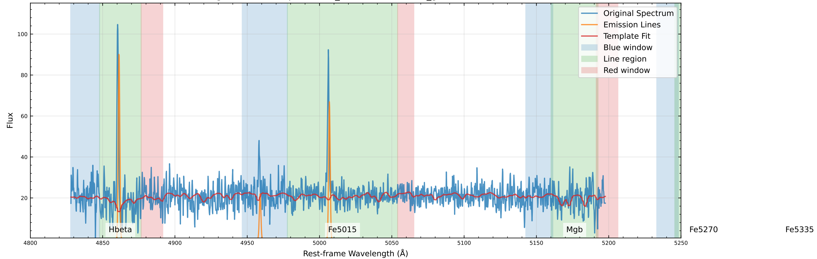
Original Data Comparison (v_star=-80.4 km/s, v_gas=-52.7 km/s)
