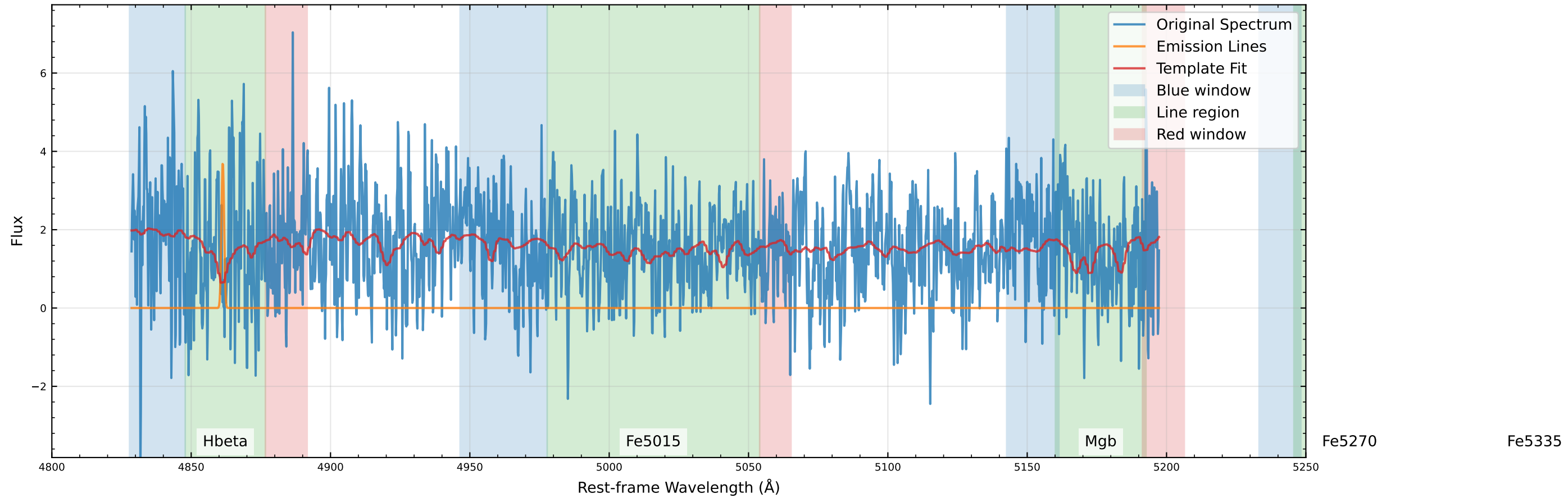
Original Data Comparison (v_star=453.9 km/s, v_gas=442.2 km/s)
