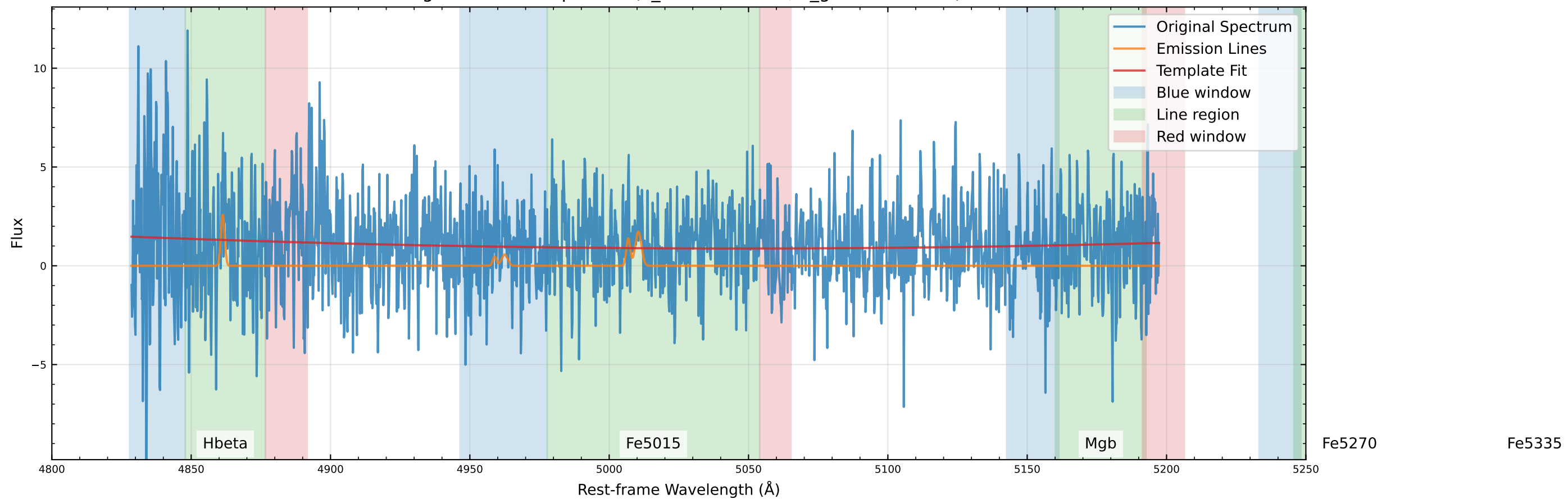
Original Data Comparison (v_star=0.0 km/s, v_gas=16.7 km/s)
