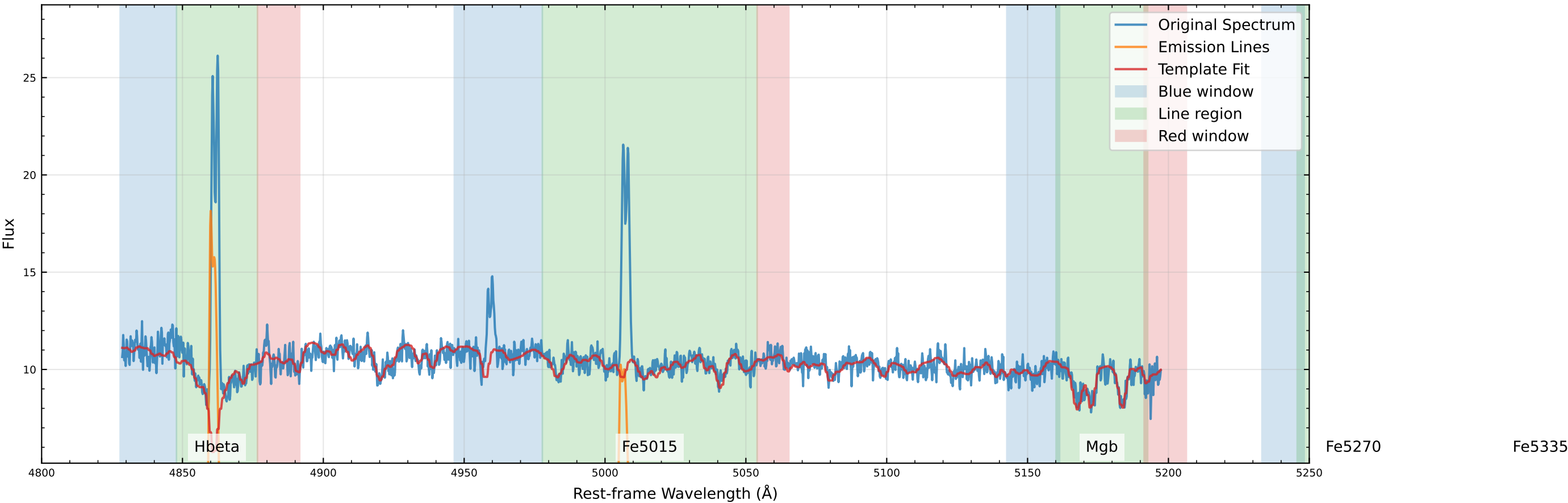
Original Data Comparison (v_star=9.8 km/s, v_gas=46.9 km/s)
