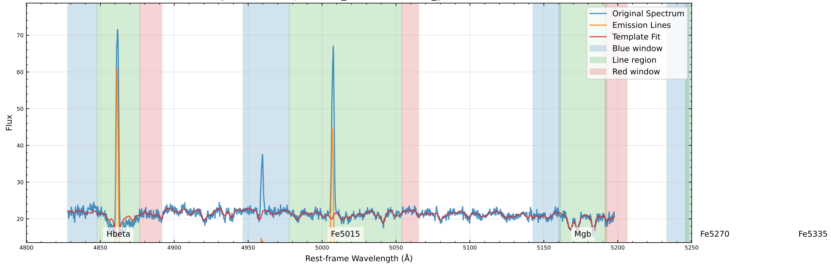
Original Data Comparison (v_star=11.3 km/s, v_gas=19.4 km/s)
