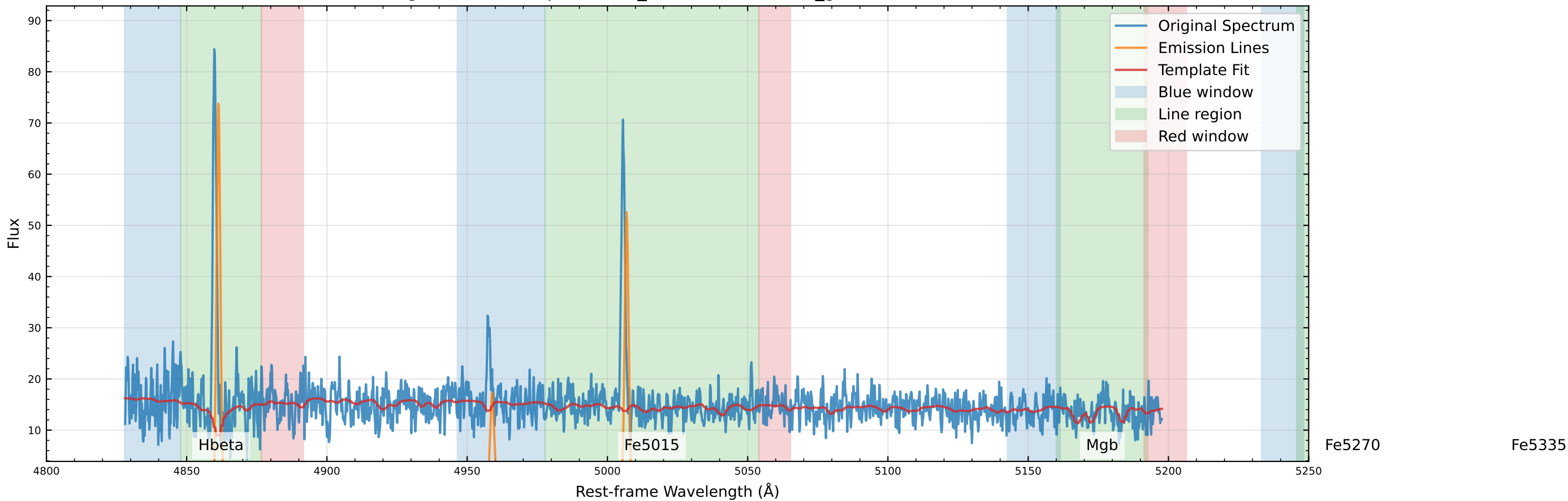
Original Data Comparison (v_star=-91.2 km/s, v_gas=-80.6 km/s)
