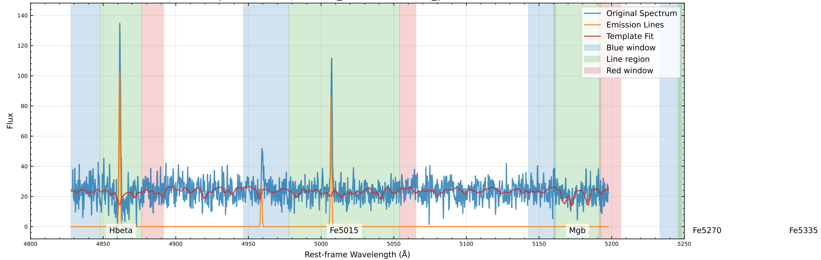
Original Data Comparison (v_star=131.4 km/s, v_gas=18.4 km/s)
