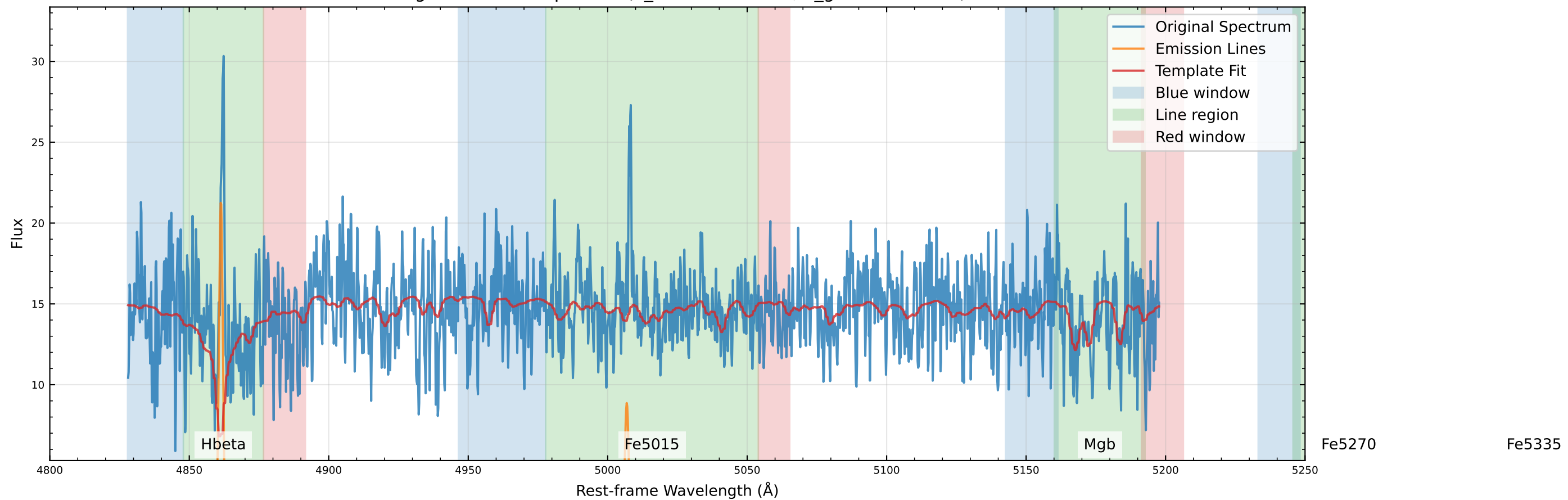
Original Data Comparison (v_star=32.3 km/s, v_gas=40.1 km/s)
