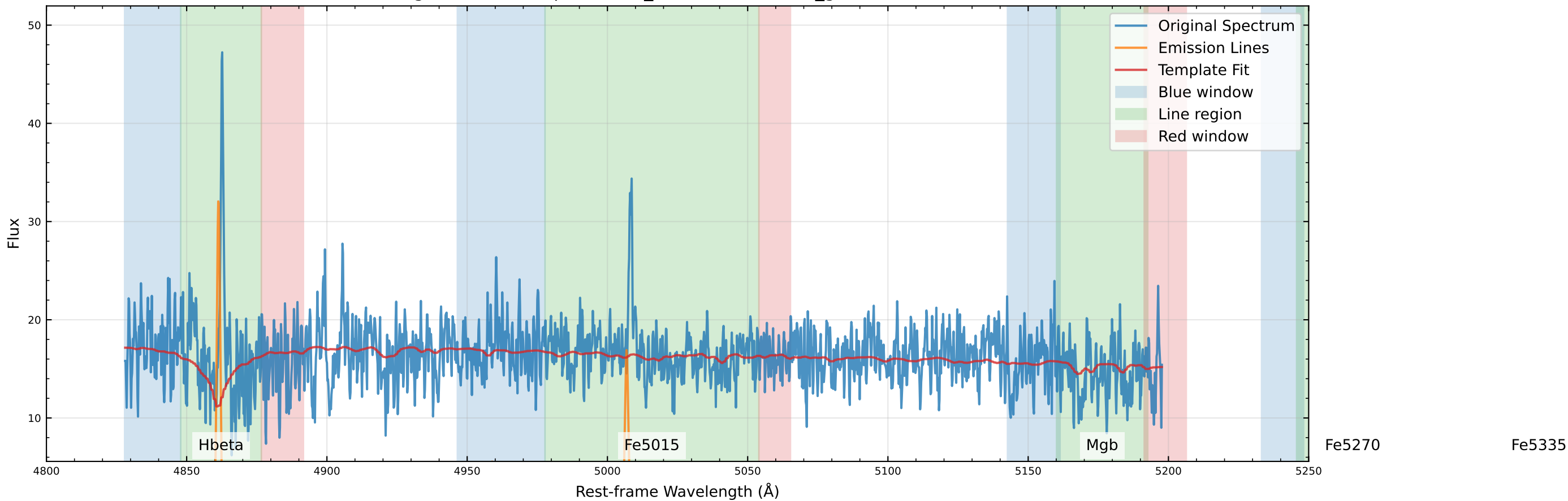
Original Data Comparison (v_star=81.3 km/s, v_gas=81.2 km/s)
