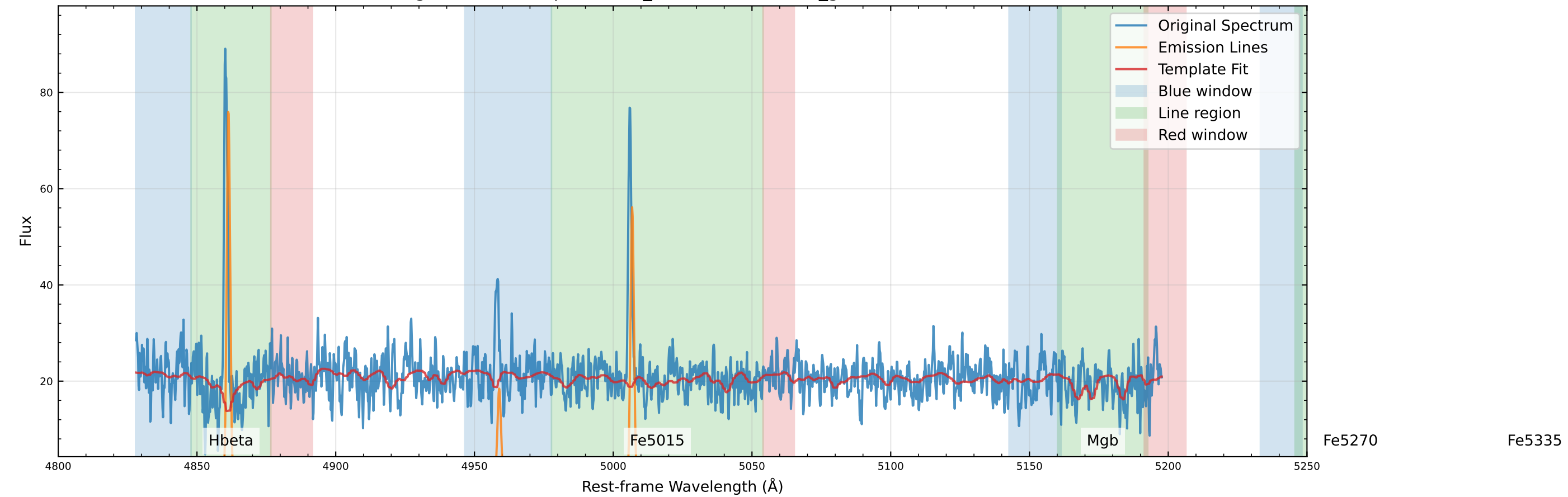
Original Data Comparison (v_star=-48.5 km/s, v_gas=-55.1 km/s)
