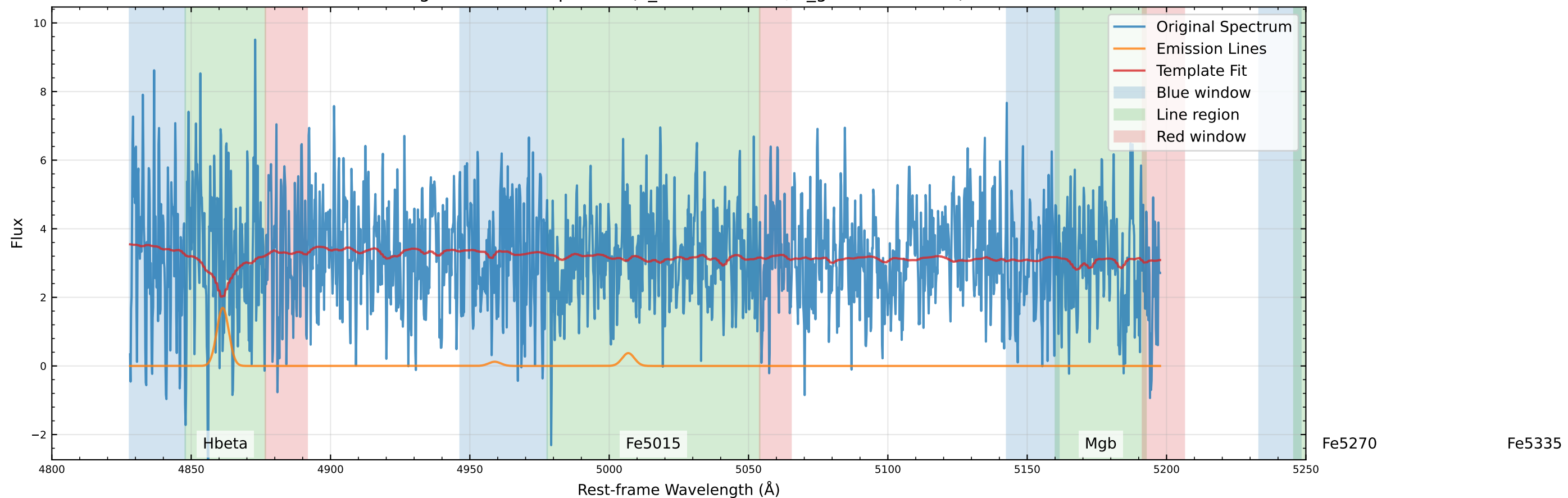
Original Data Comparison (v_star=7.1 km/s, v_gas=-25.0 km/s)
