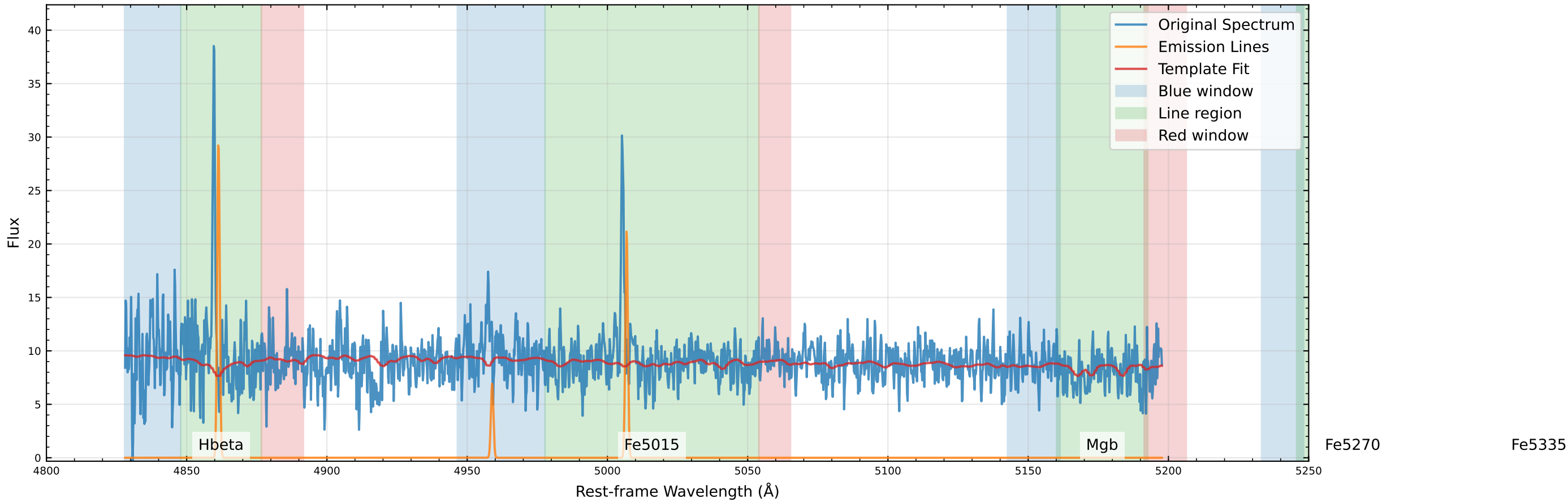
Original Data Comparison (v_star=-98.9 km/s, v_gas=-98.4 km/s)
