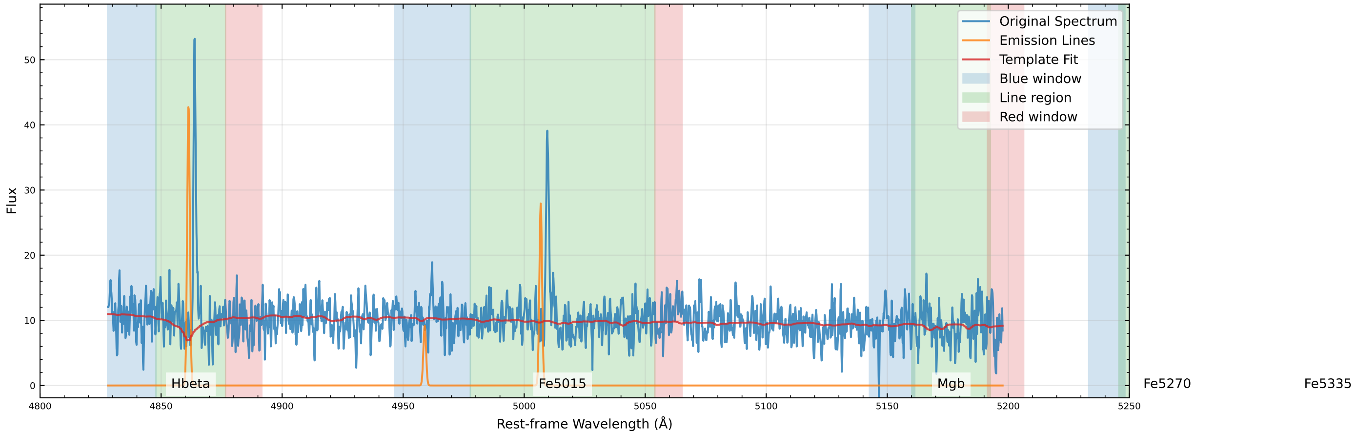
Original Data Comparison (v_star=146.5 km/s, v_gas=161.3 km/s)
