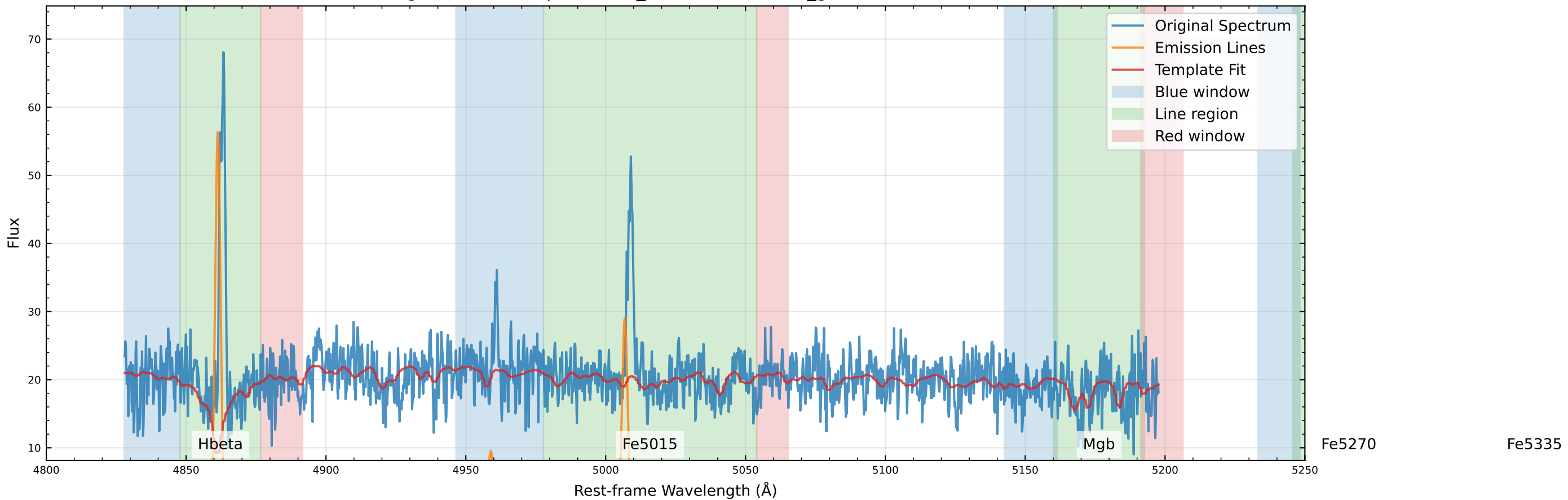
Original Data Comparison (v_star=88.3 km/s, v_gas=104.9 km/s)
