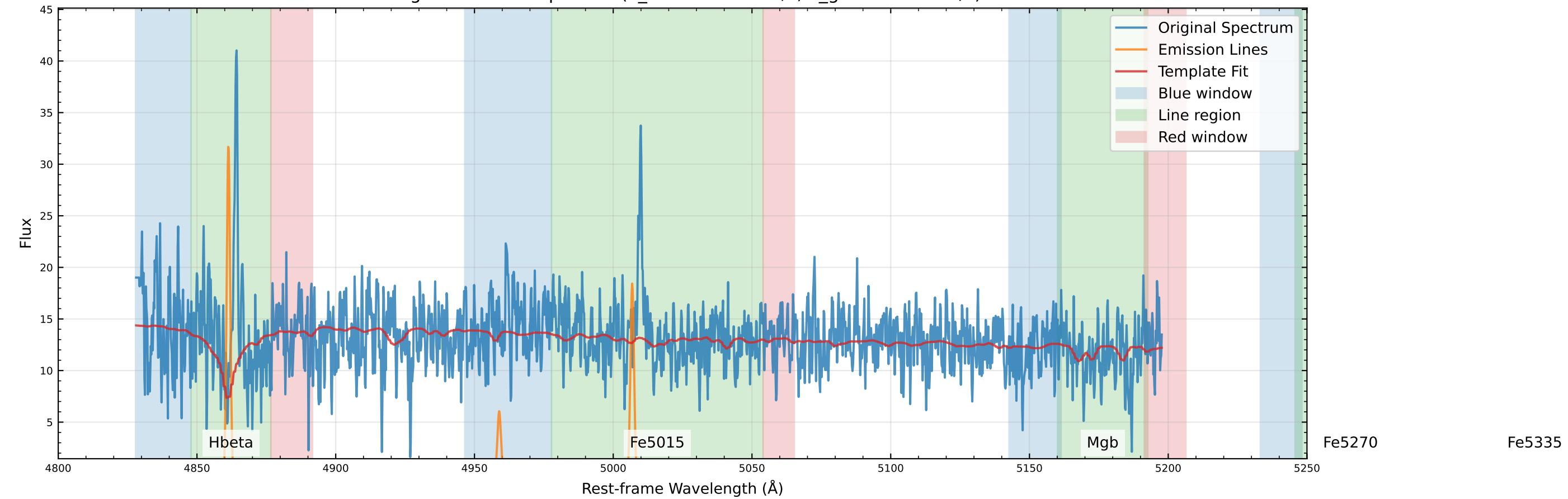
Original Data Comparison (v_star=166.5 km/s, v_gas=170.1 km/s)
