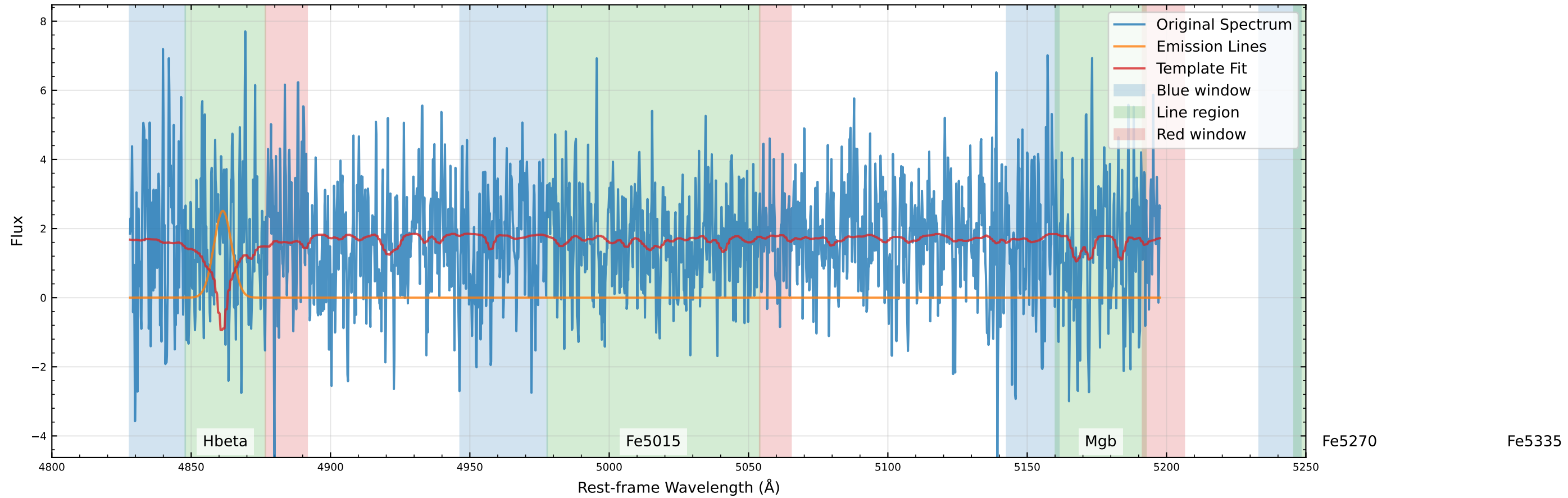
Original Data Comparison (v_star=-230.3 km/s, v_gas=-208.4 km/s)
