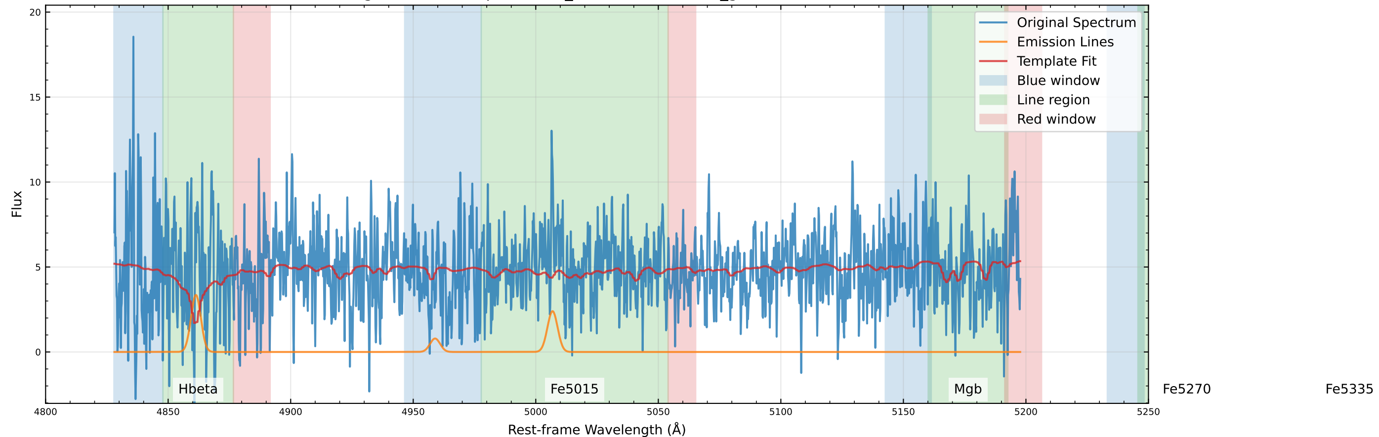
Original Data Comparison (v_star=-68.2 km/s, v_gas=19.0 km/s)
