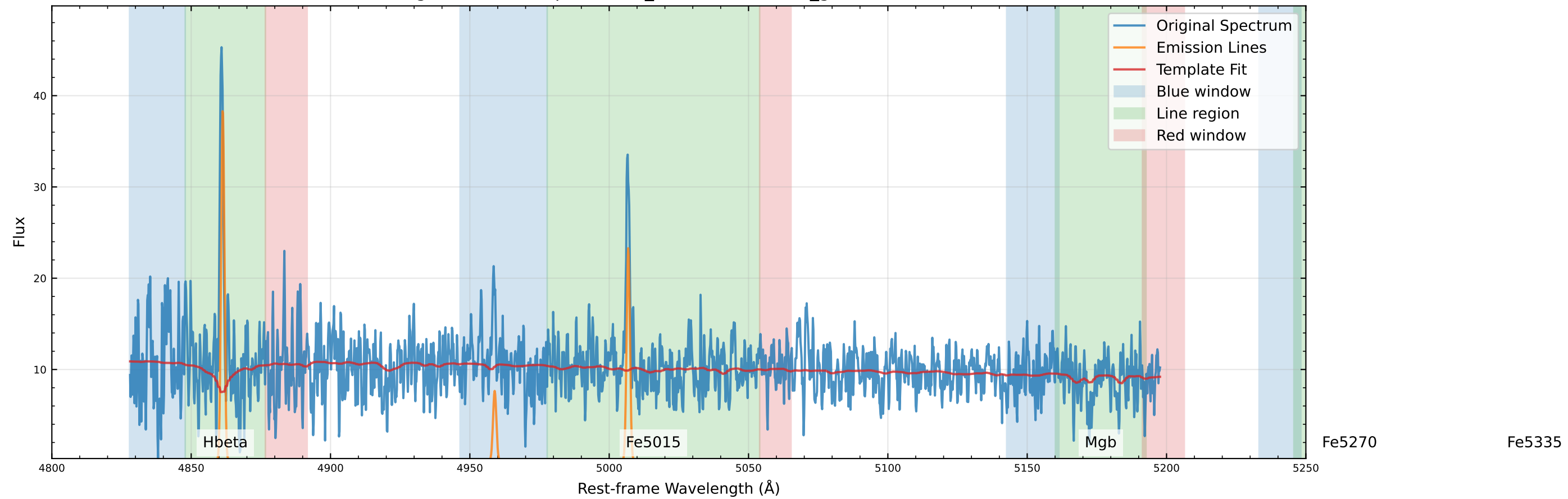
Original Data Comparison (v_star=-3.1 km/s, v_gas=-22.8 km/s)
